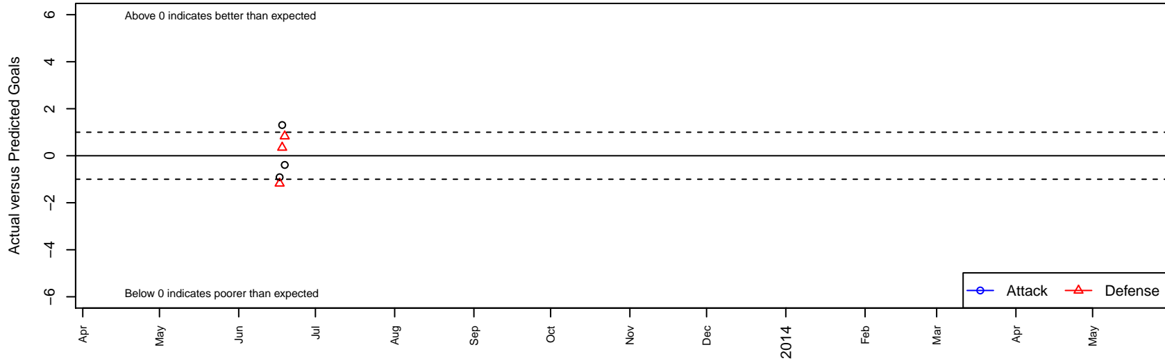
Peninsula SC Extreme B94 Dots are actual minus expected GF (blue circles) and GA (red triangles). Blue line is smoothed change in attack strength. Red is smoothed change in defense strength.
